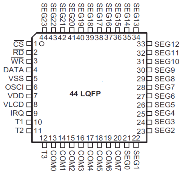
LQFP44
